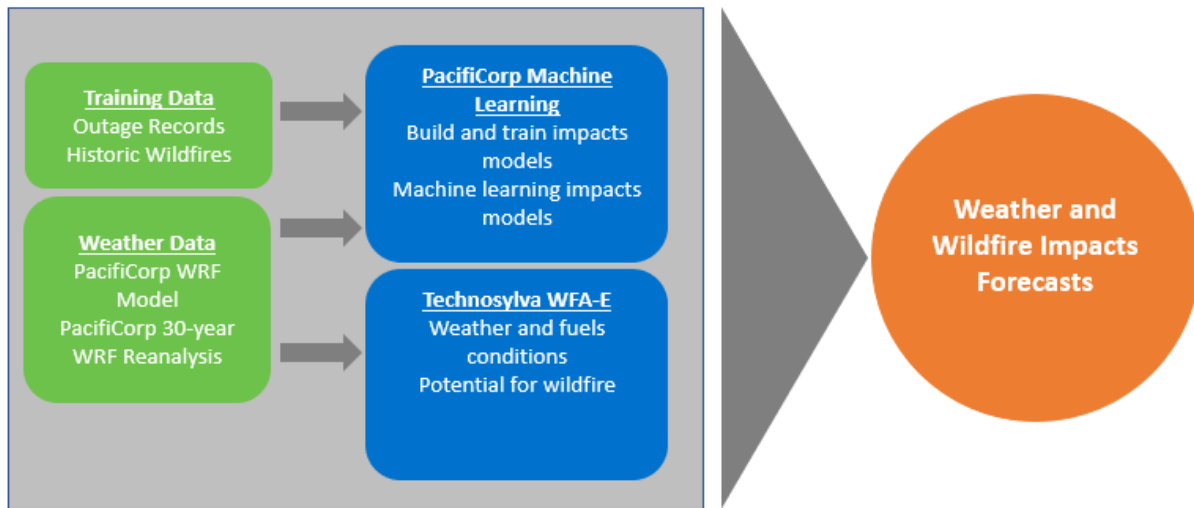
Figure PAC 10-17: Existing Operational Weather and Seasonal Wildfire Modeling Approach
