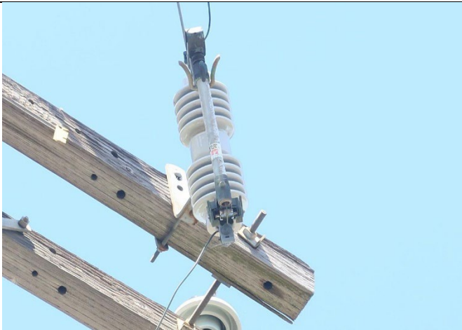
Item1IA1Img4: Close-up view of non-exempt expulsion fuse
