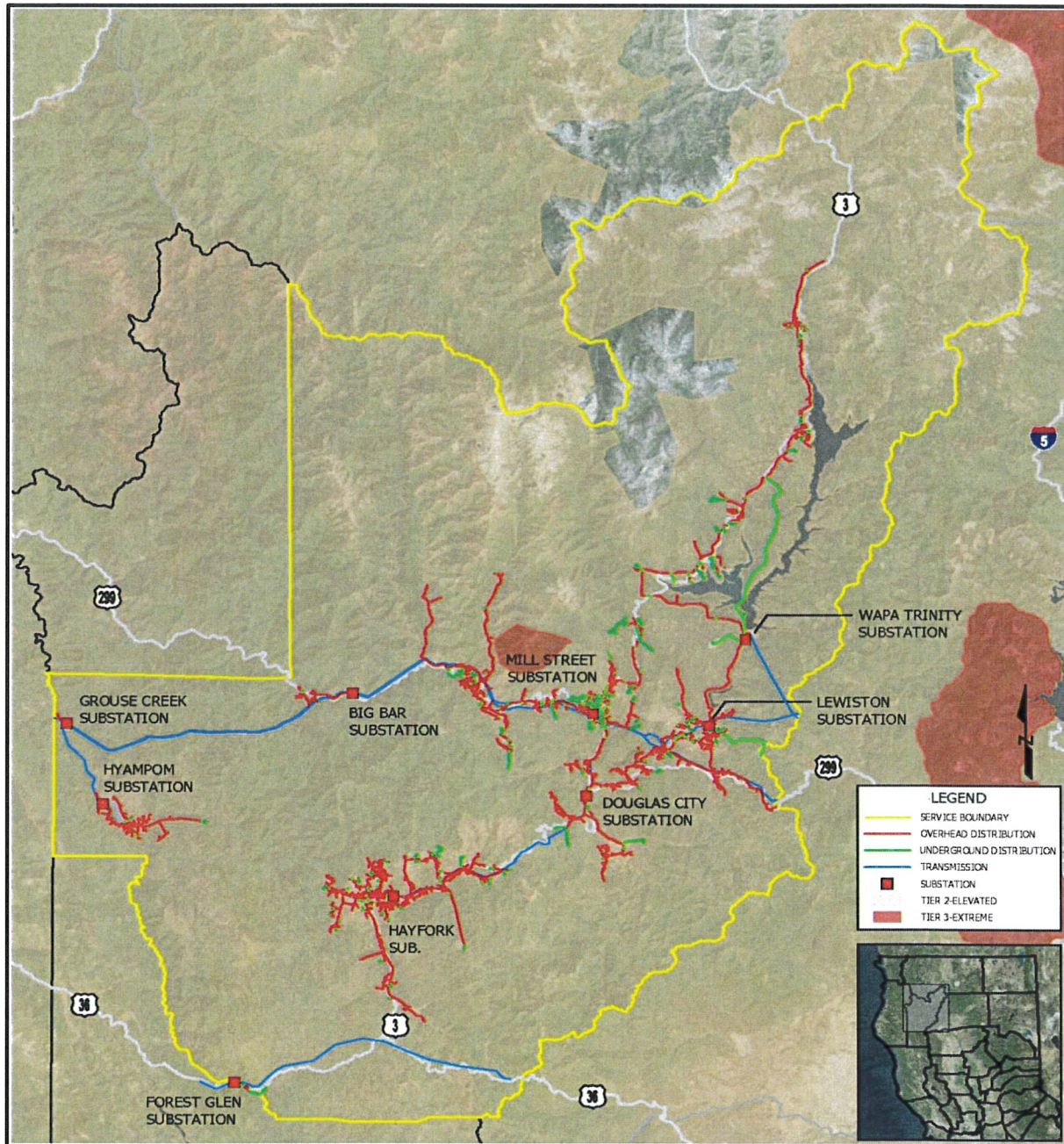
Figure 3. A high-level diagram of TPUD assets in relation to the threat level tiers. As illustrated, most of TPUD's T&D lines and substations are in "Tier 2 – Elevated" fire-threat areas. Portions of the distribution system are located outside of the High Fire-Threat Districts, as well as three substations.
