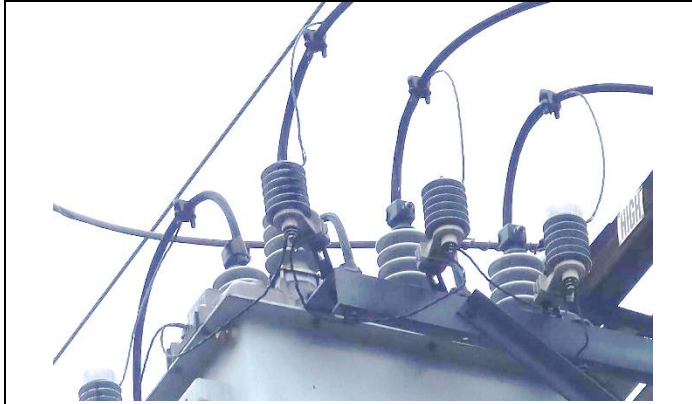
Item1IA1Img3: CAL FIRE-approved lightning arresters not installed
