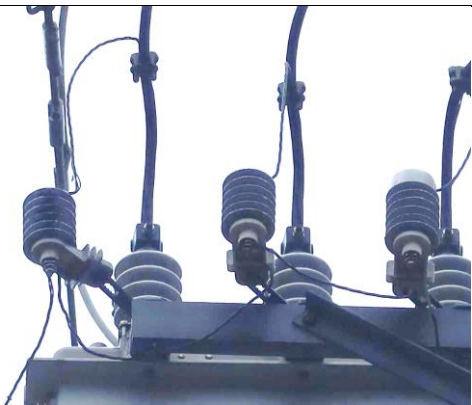
Item1IA1Img2: CAL FIRE-approved lightning arresters not installed
