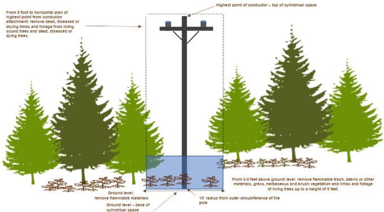
Figure 8- 15 12 Pole Clearing
