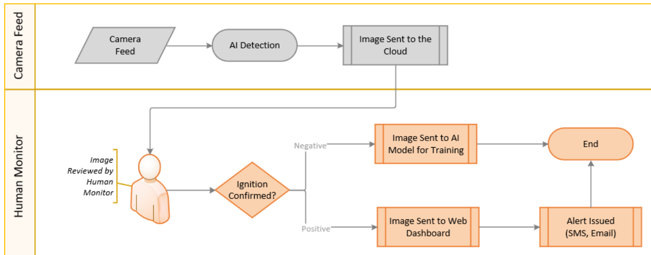
Figure 8-208-16: Camera Data Flow Diagram
