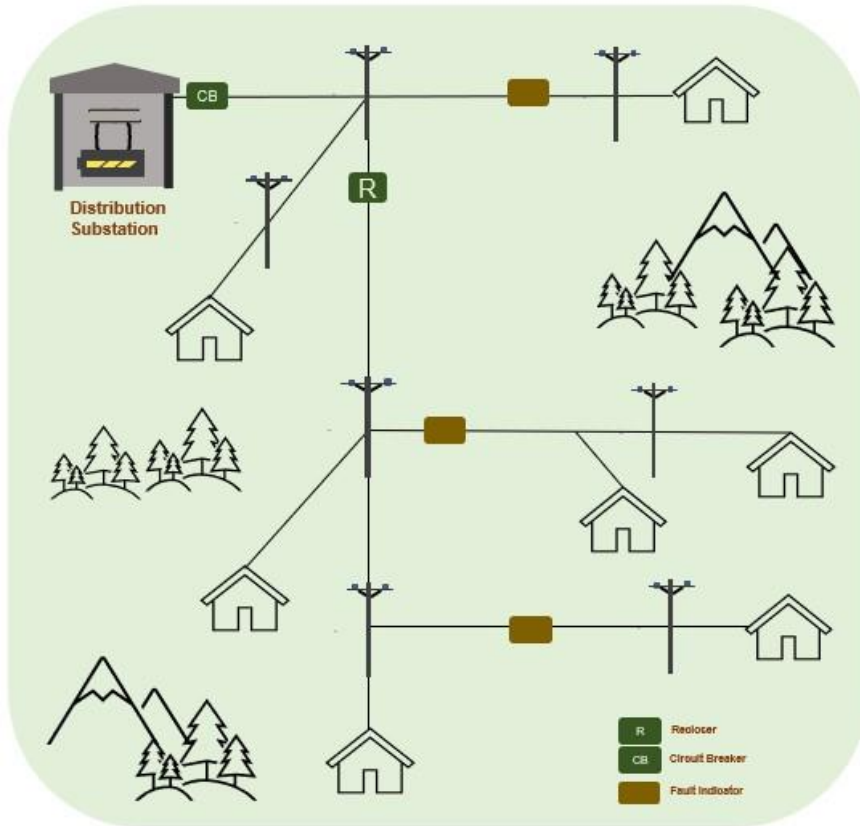
Figure 8-128-10 Figure 8-128-12: General Fault Indicator Location
