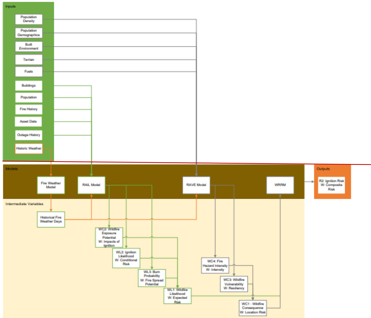
Figure 6-9:6-9 FireSight WRRM Calculation Schematic
