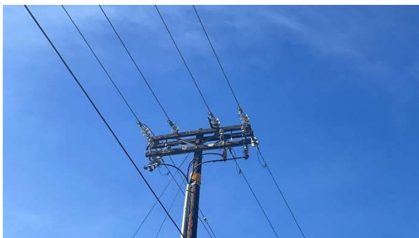
Item1IA1mg1: Avian protection is dislodged on the center phase, no other avian protections visible
