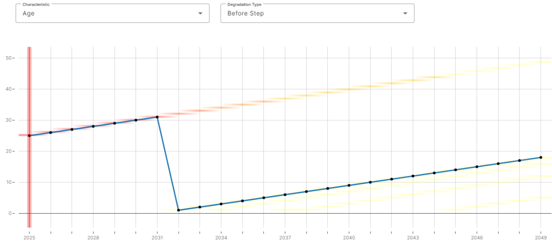
Figure 15. Degradation of the age characteristic of the selected conductor asset over the 5th iteration of the simulation. The other colored lines represent a heat map of the degradation curves observed in the other iterations.
