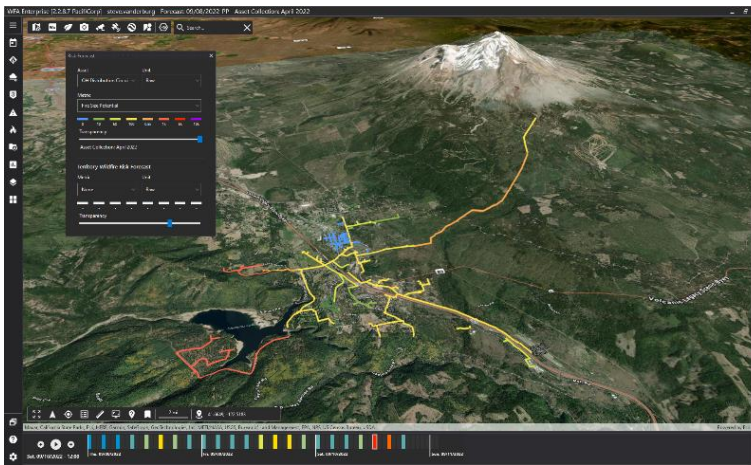
Figure 8-18 Example of FireCast Output, Mt. Shasta
