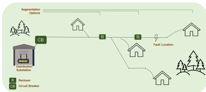
Figure 8-7: Example of Distribution Circuit with Multiple Reclosers
