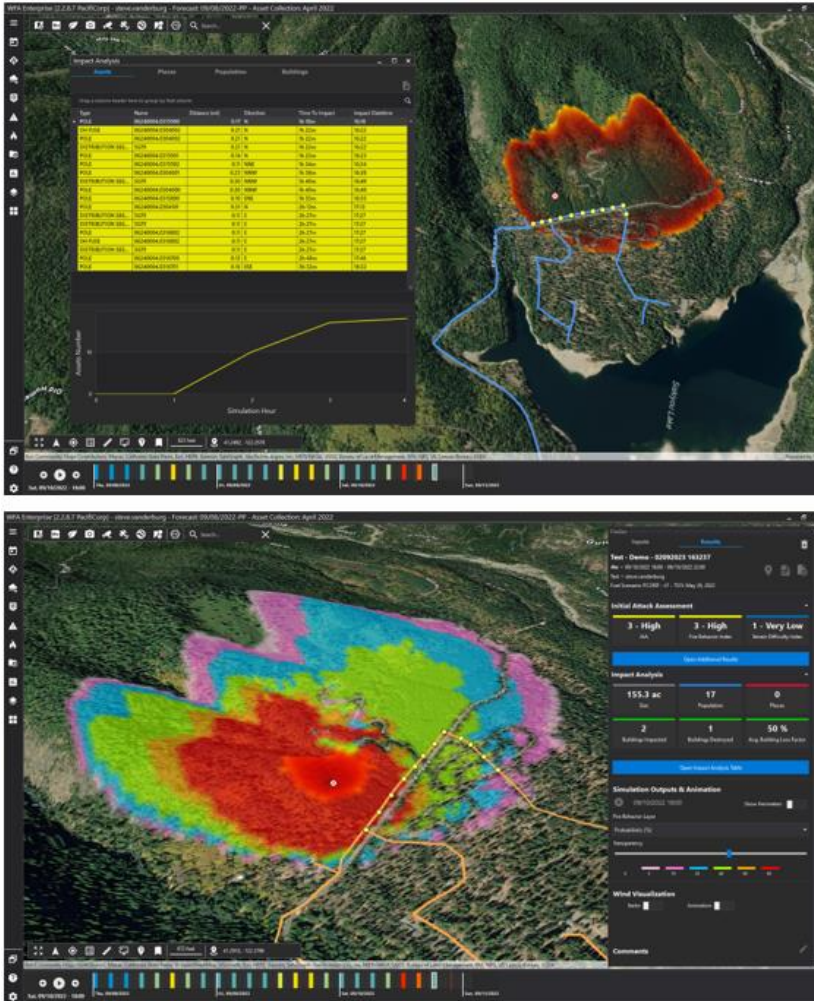
Figure 8-17 Example of a FireSim Output, Mt. Shasta
