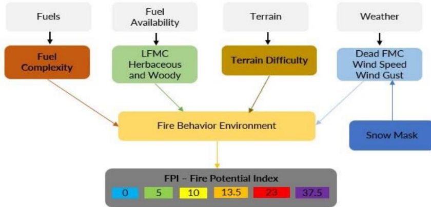
Figure 8-27 2023 Fire Potential Index (FPI) Model
