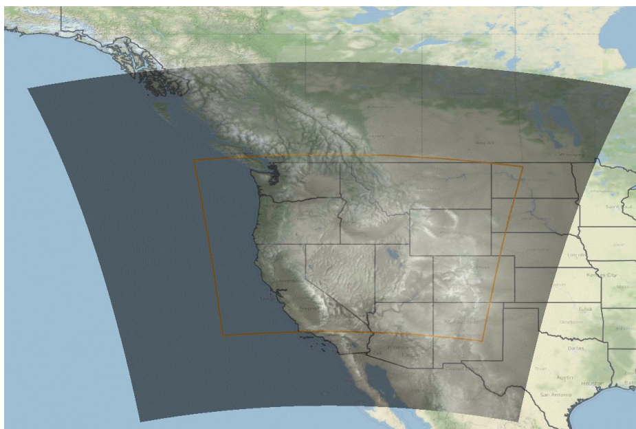
Figure 8-24 Pacific Power WRF Domain
