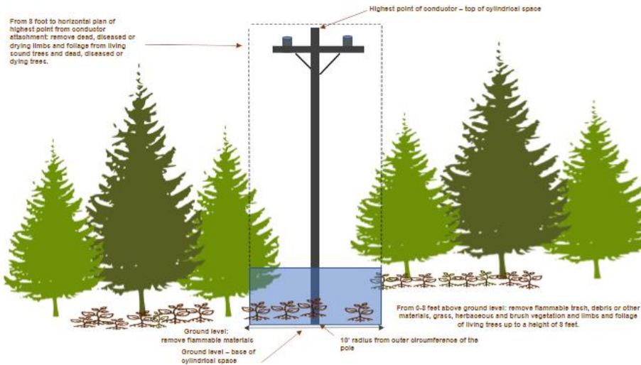
Figure 8-12 Pole Clearing
