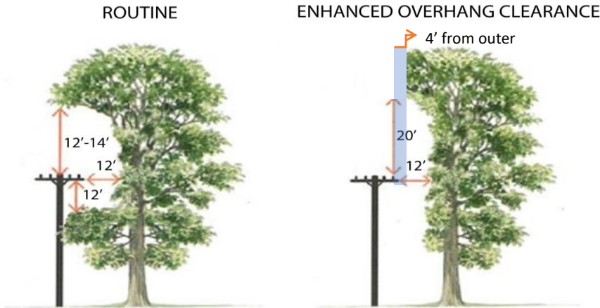
Figure 8-13 Enhanced Overhang Clearance
