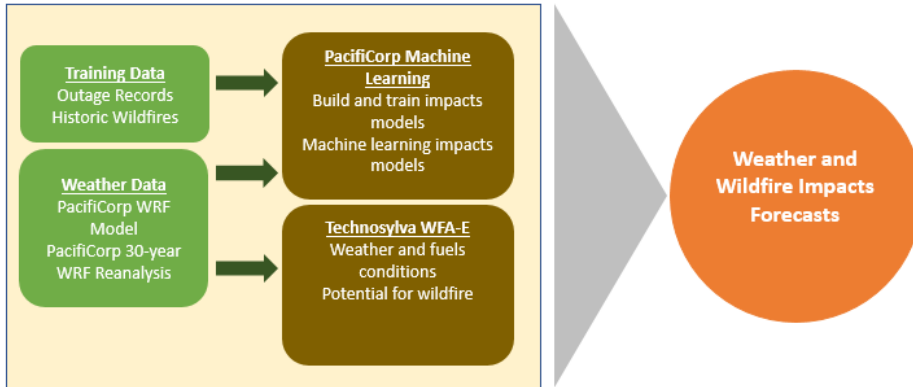
Figure 8-23 Existing Weather and Seasonal Wildfire Modeling Approach
