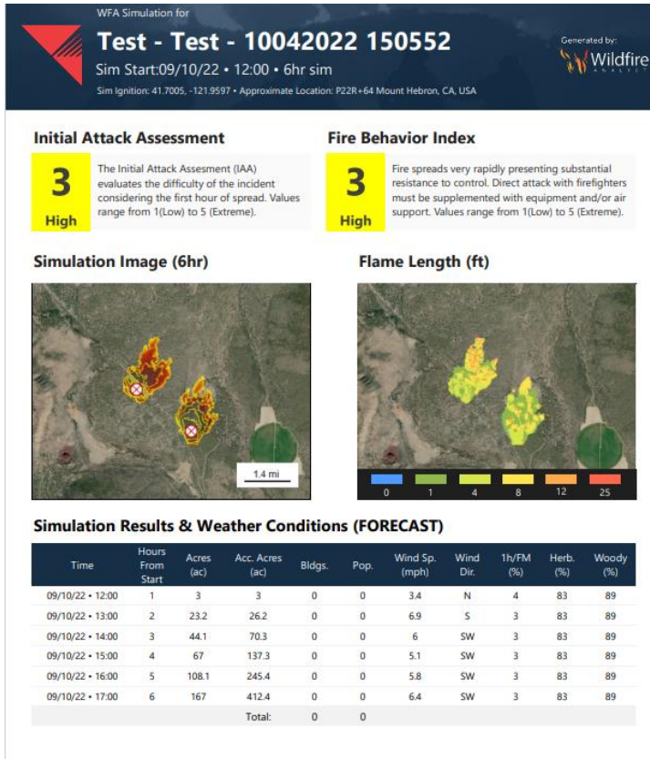
Figure 8-19: Example of FireSim Summary Report
