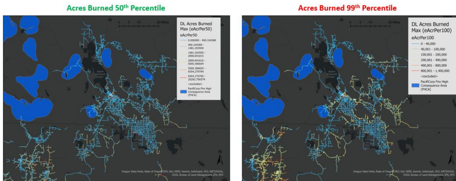
Figure B-6. Example of WRRM Output
