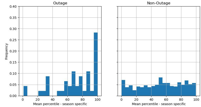
Outage v/s non-outage wind speed mean %ile - autumn
