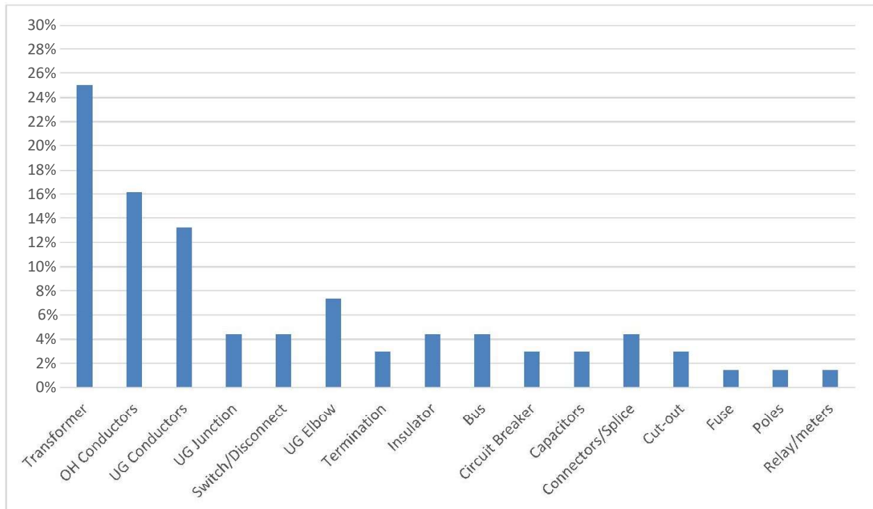
Figure 2. Outages Based on GWP Equipment (2013-2023)
