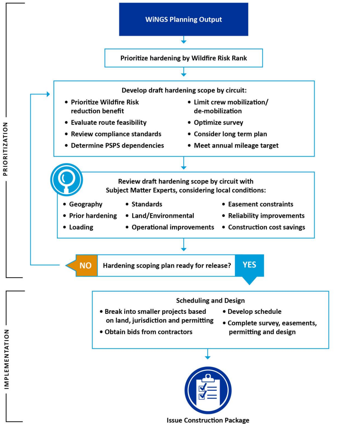
Figure 7-4: High-Level Mitigation Prioritization to Reduce Wildfire and PSPS Risk
