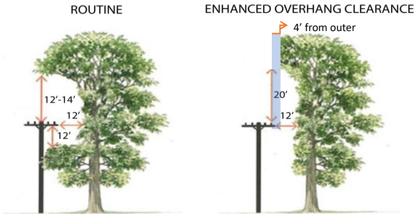
Figure 8-13 Enhanced Overhang Clearance
