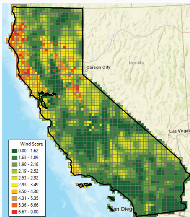
Figure 3.16. Raster Map for Wind Scores Using the Comprehensive Wind Score Model
