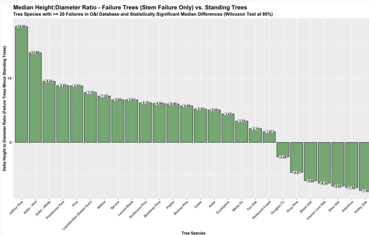
FIGURE F3. Comparison of statistically significant ( p < 0.05 ) failure tree to standing tree median height to diameter ratios.
