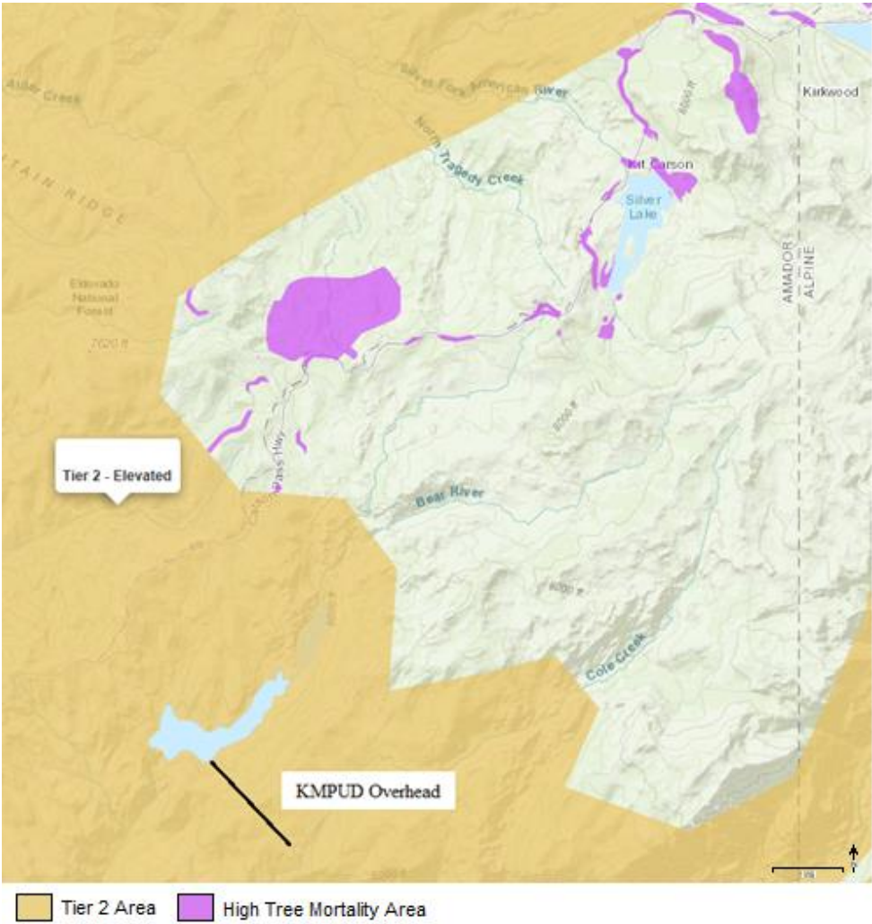
Figure 2 – Overlay KMPUD Overhead Transmission Line
