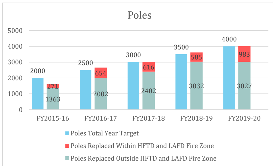
Graph 1: PSRP Pole
