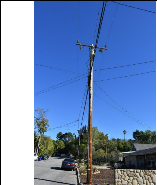
G1mg3: View of pole with bare conductor
