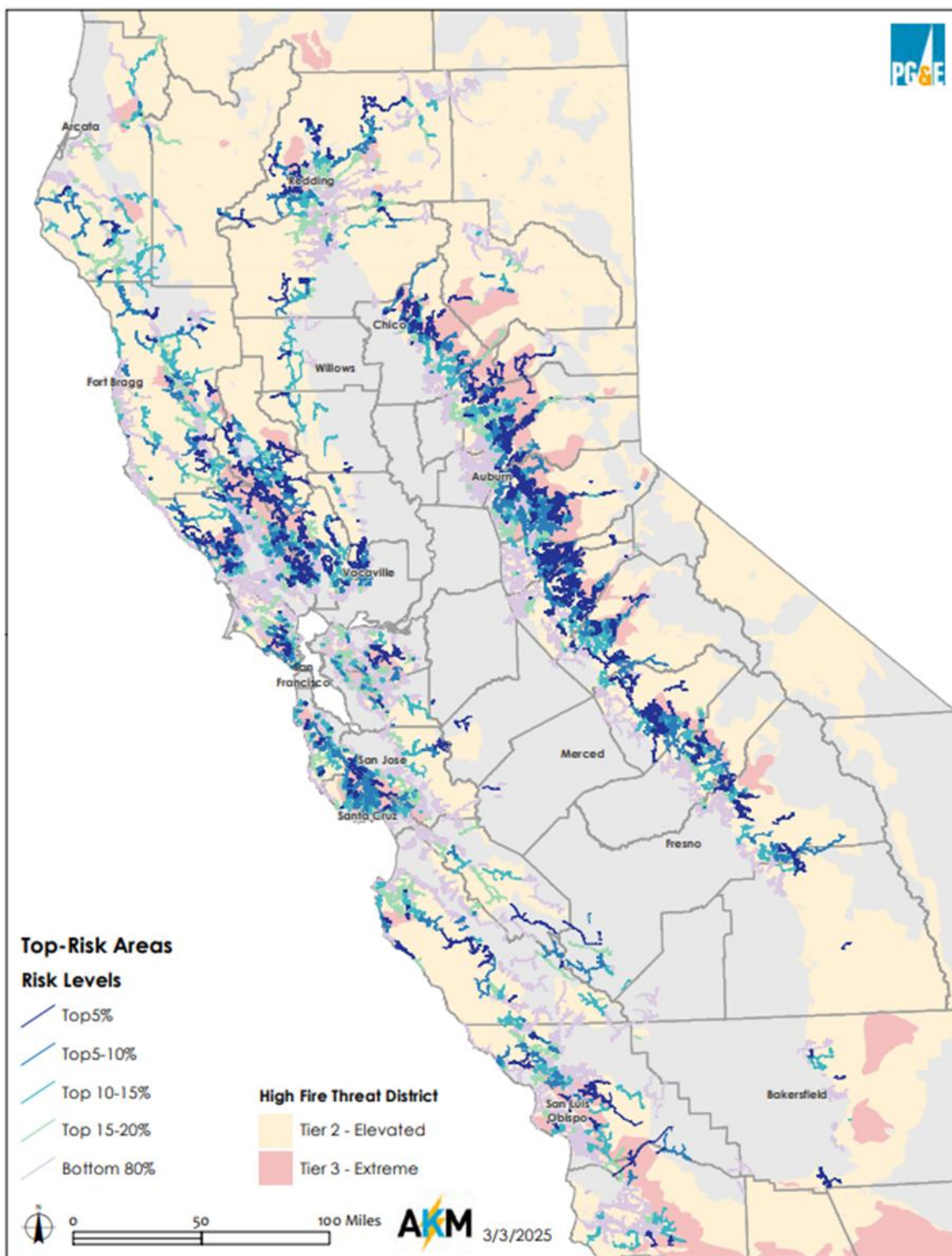
FIGURE PG&E-5.5.1.1-1: WDRM v4 HFRA CIRCUIT SEGMENT RISK MAP
