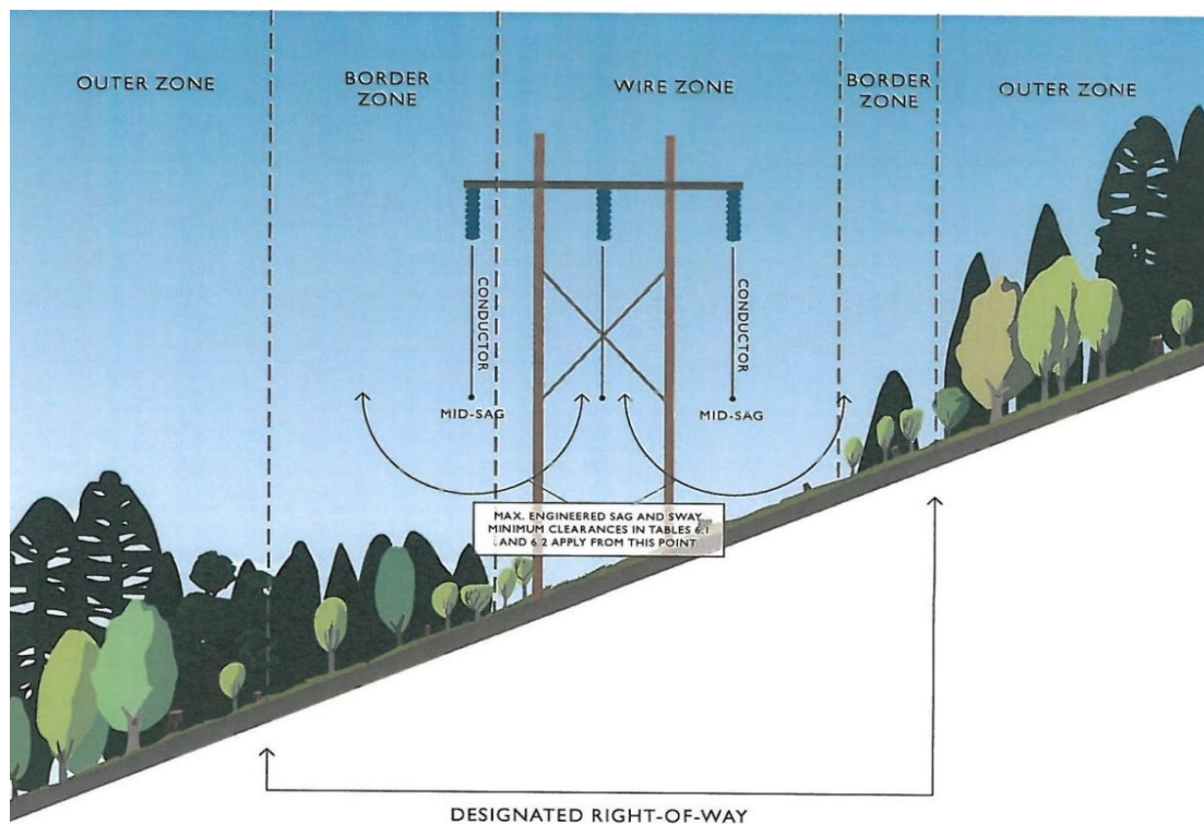
Figure 3.10. The border zone is condensed on upslopes, where wire sag and sway could bring it into contact with trees and is extended on downslopes.
