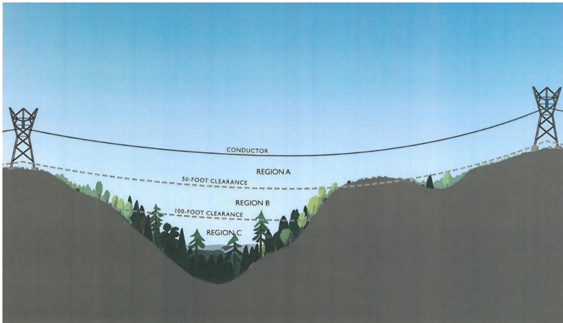
Figure 3.11. Transmission under-clearance regions.
