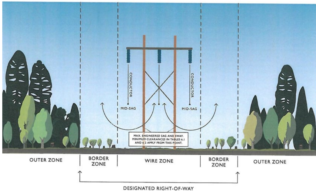
Figure 3.9. Bramble and Byrnes wire zone-border zone (adapted from Bramble et al. 1985; Yahner et al. 2004).
