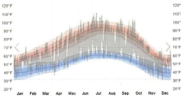
Temperature history in 2024 in Roseville
