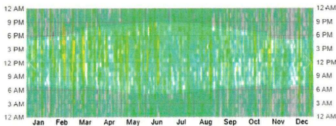
Hourly Wind Speed in 2024 in Roseville
