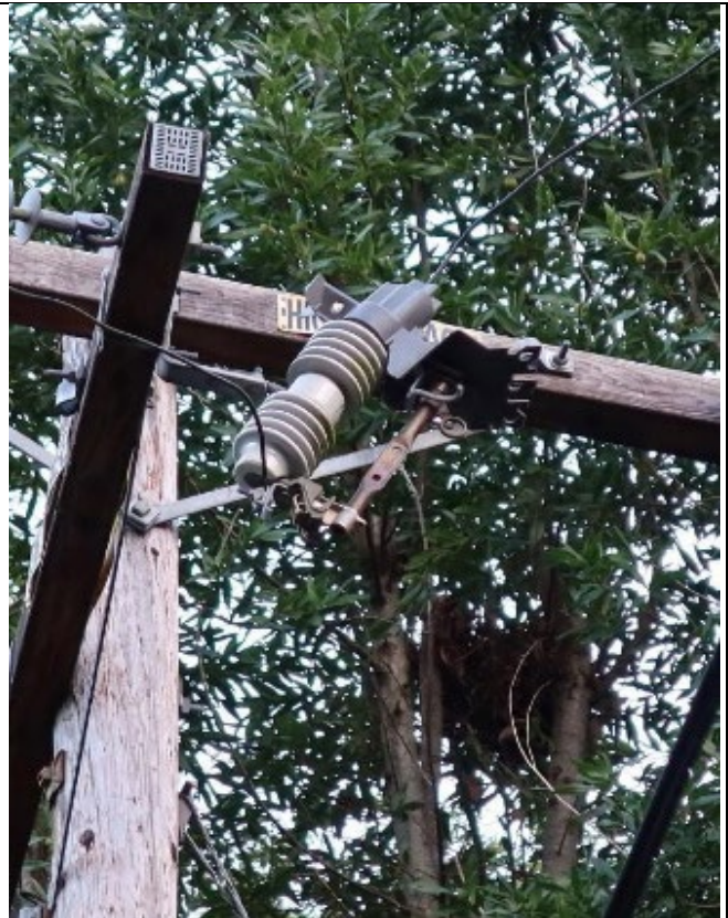
IA1Img2: Solid blade disconnect one.
